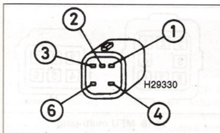
14.13 Stepper motor multi-plug pin numbers
