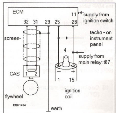
14.9 Typical local wiring diagram: ignition
