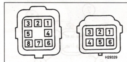
14.18 MFU multi-plug
