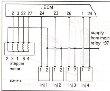
14.12 Typical local wiring diagram: injectors, stepper motor
