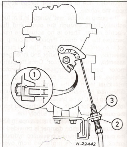
14.8 Adjust the throttle lost motion gap - see text
