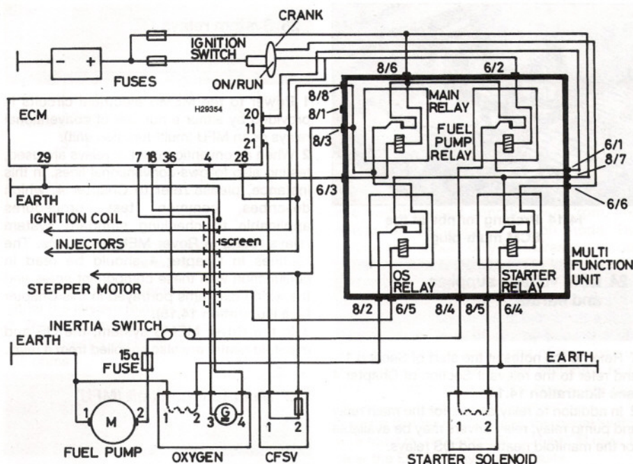
14.16 Typical local wiring diagram: relays (MFU) and components
