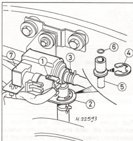
14.7 Carbon filter solenoid valve (CFSV)
