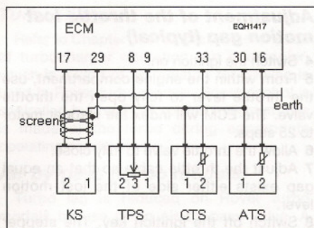
14.10 Typical local wiring diagram: sensors
