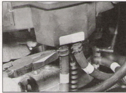
14.2 SPI: The MAP sensor vacuum hose connections to the fuel trap at the air filter. The hoses are colour coded to ensure correct refitting
