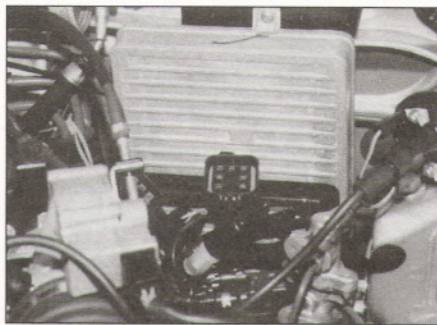
14.4 Rover 820 MEMS multi-function unit (MFU)
