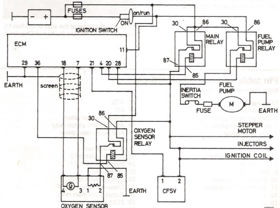
14.15 Typical local wiring diagram: relays and components
