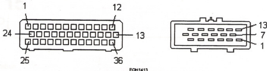
14.19 Typical 36-pin and 18-pin multi-plugs
