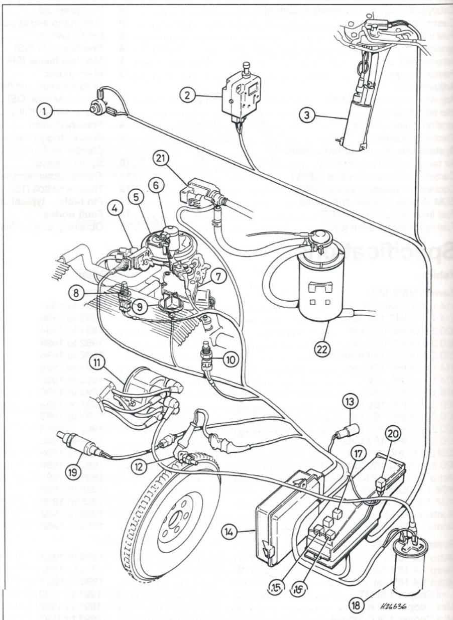
14.1 Rover MEMS (Rover 214 SPI). Multi-point systems are very similar
