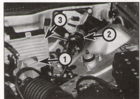
14.3 Rover 820 stepper motor 1 Stepper motor 2 Ignition coil 3 ECM
