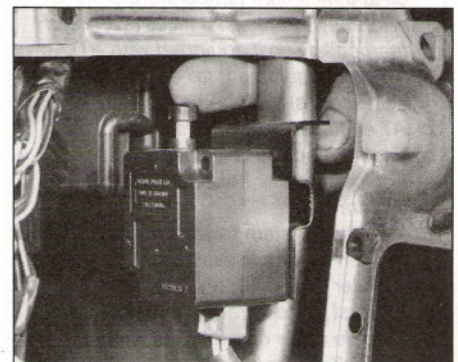
14.6 Reset inertia switch by depressing plunger
