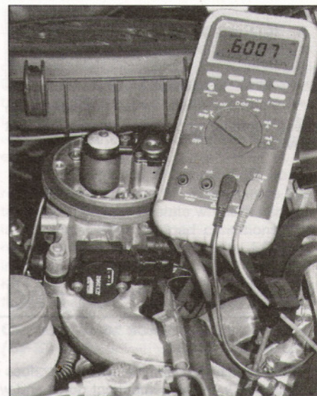
14.11 Check the throttle pot voltage output with the aid of a voltmeter
