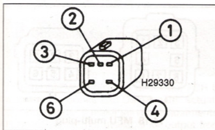
14.13 Stepper motor multi-plug pin numbers
